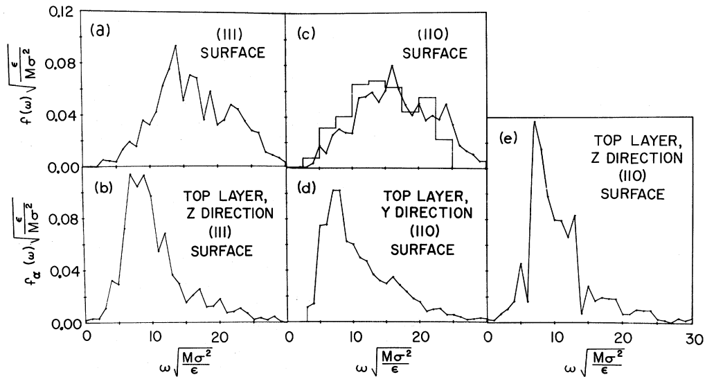
FIG. 25. Frequency distribution functions f(\omega) and effective frequency distribution functions at surface, f_{\alpha}(\omega) , calculated in molecular dynamics computer experiments. (a) f(\omega) for 11-layer crystal with (111) surfaces. (b) f_{\alpha}(\omega) for (111) surface. (c) f(\omega) for 11-layer crystal with (110) surfaces. The histogram was calculated for the same model using lattice dynamics rather than molecular dynamics. (d) f_{\alpha}(\omega) for (110) surface. (e) f_{\alpha}(\omega) for (110) surface. All of these results were obtained with 11-layer crystals at a density corresponding to \sigma/a=1.28 . The temperatures were given by k_B T/\epsilon = 0.369 for (a) and (b), and by k_B T/\epsilon = 0.335 for (c), (d), and (e).
