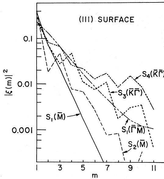
FIG. 9. Squared amplitude |\bar{\xi}(m)|^2 vs layer number m for the surface modes shown in Fig. 8. Here m=1 for a surface layer and m=11 for the center layer. The vertical scale is logarithmic. The mode S_1(\bar{\Gamma}\bar{M}) is that mode on the S_1 branch which lies halfway between \bar{\Gamma} and \bar{M} in Fig. 8. The modes S_3(\bar{K}\bar{\Gamma}) and S_4(\bar{K}\bar{\Gamma}) lie on the S_3 and S_4 branches, respectively, just to the right of \bar{K} in Fig. 8. S_1(\bar{M}) and S_2(\bar{M}) lie on the S_1 and S_2 branches, respectively, at the point \bar{M} .
