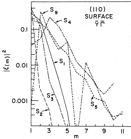
FIG. 15. Graph of |\bar{\xi}(m)|^2 for surface modes S_1 , S_2 , S_3 , S_4 , S_5 , and S_9 at a point along \bar{Y}\bar{T} just to the right of \bar{Y} in Fig. 13.
